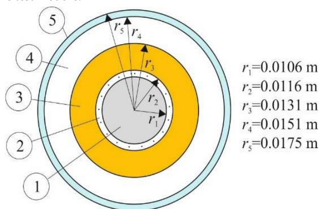
Figure 2. A cross-section of the test module: 1 – cartridge heater, 2 – thermally conductive filler with thermocouples, 3 – copper tube, 4 – minigap with HFE-649 fluid, 5 – glass tube (schematic drawing, not to scale).
