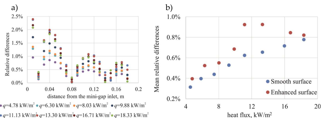
Figure 4. (a) Relative differences for the enhanced-surface temperature as a function of distance from the minigap inlet; (b) mean relative differences for both analysed surfaces as a function of heat flux.
